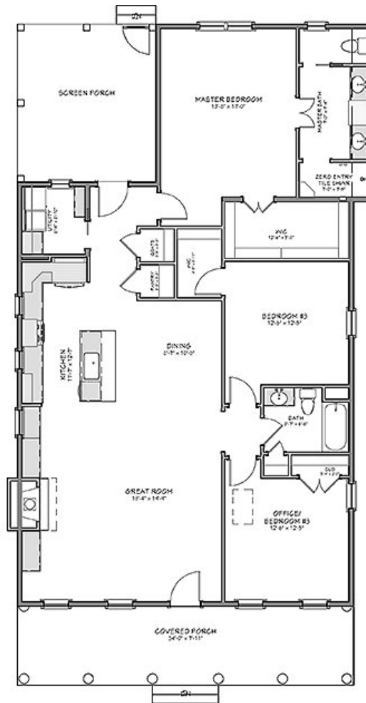
THE CALHOUN COTTAGE VARIATION 1524 sq ft
