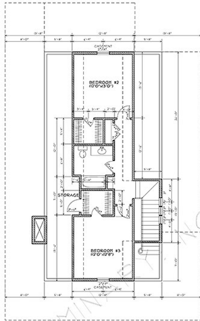
SECOND FLOOR PLAN * 9' CEILING HT.
