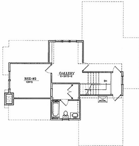
2ND FLOOR PLAN SCALE: 1/8"=1'-0"
