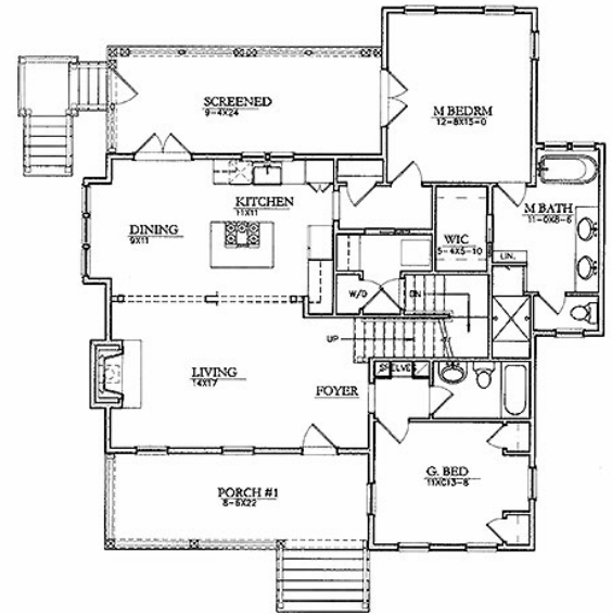
1ST FLOOR PLAN SCALE: 1/8"=1'-0"
