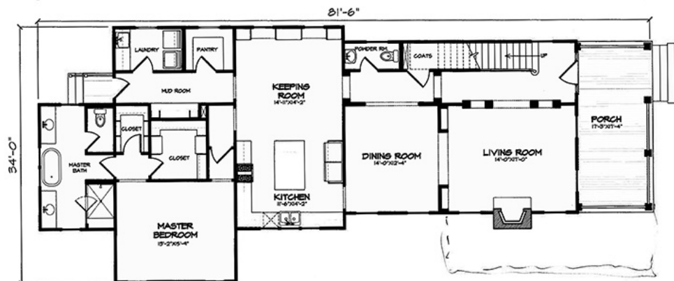
① FIRST FLOOR PLAN
